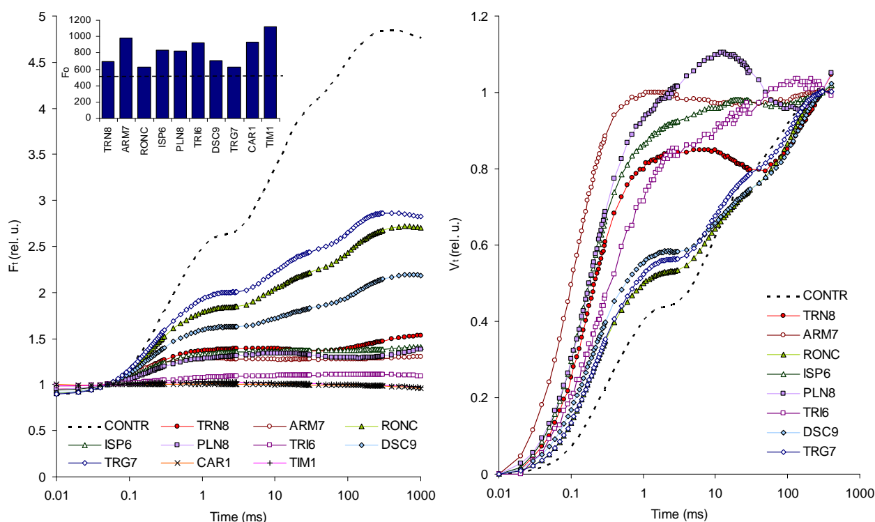
Figure 3: a) The rapid chlorophyll fluorescence kinetics in heat-stress exposed plants of wheat genotypes compared to average curve in non-stressed plants (CONTR; short-dashed line). The curves are shown with normalised F_0 . The observed F_0 values are shown in small graph above the curves (the short-dashed line shows average F_0 value in non-stressed plants). b) The graph of relative variable fluorescence ( V_t ) observed in heat-stressed samples compared to average non-stressed curve (CONTR, short-dashed line).
