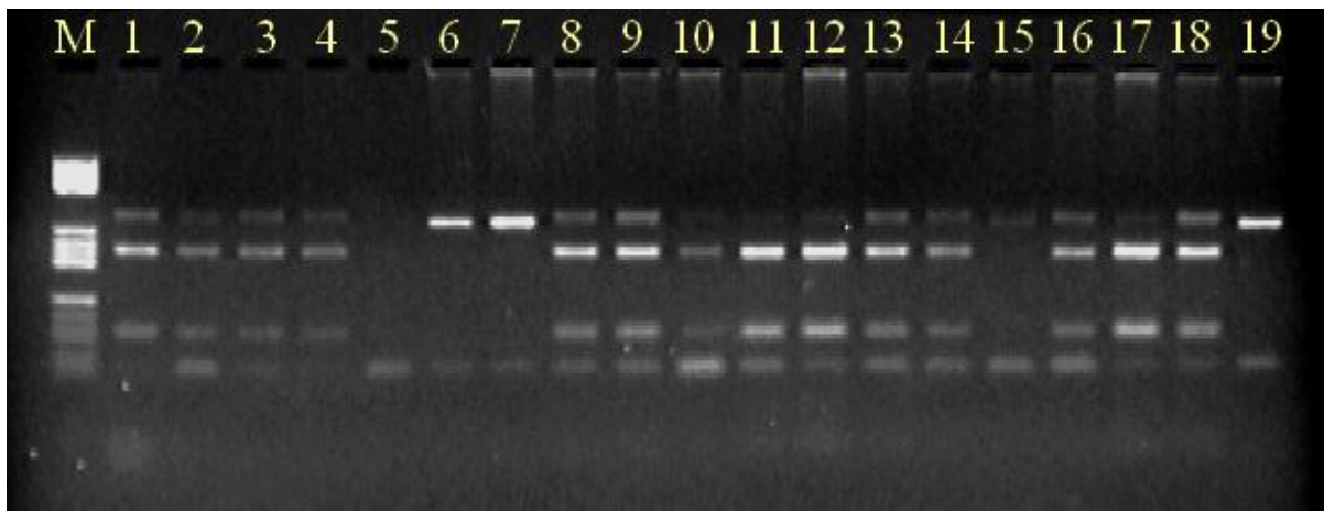
Figure 1. PRL gene genotype identification (molecular M marker pBR322 DNA/BsuRI; genotypes: Del/Del – 6,7,15,19; Ins/Del – 1,2,3,4,8,9,13,14,16,18; Ins/Ins – 10,11,12,17).
