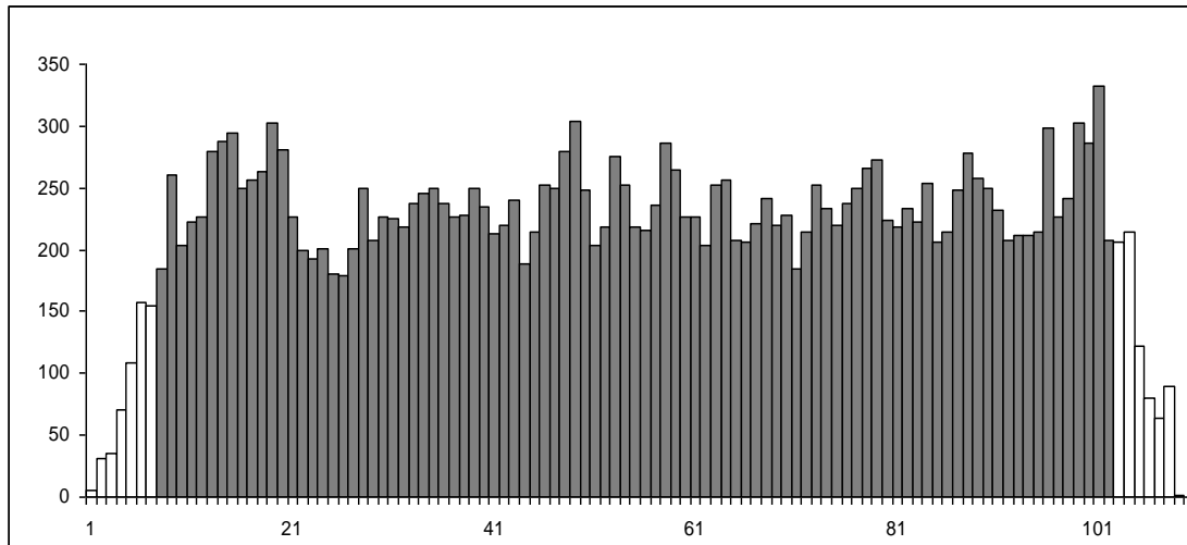
Figure 3. Liquid volumes in grooves of manual table calculated for 20 nozzles tested on the electronic table. The nozzle order (9,12,8,5,10,17,6,15,1,14,16,20,7,19,13,11,2,18,3,4).
